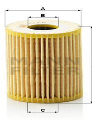
Oil Filter HU 610 x EM-10118
